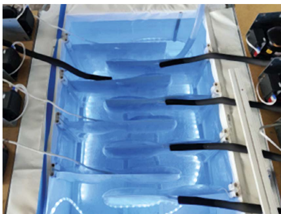
Figure 4.8 Ice-based thermal storage with separate evaporators and cooling units.
