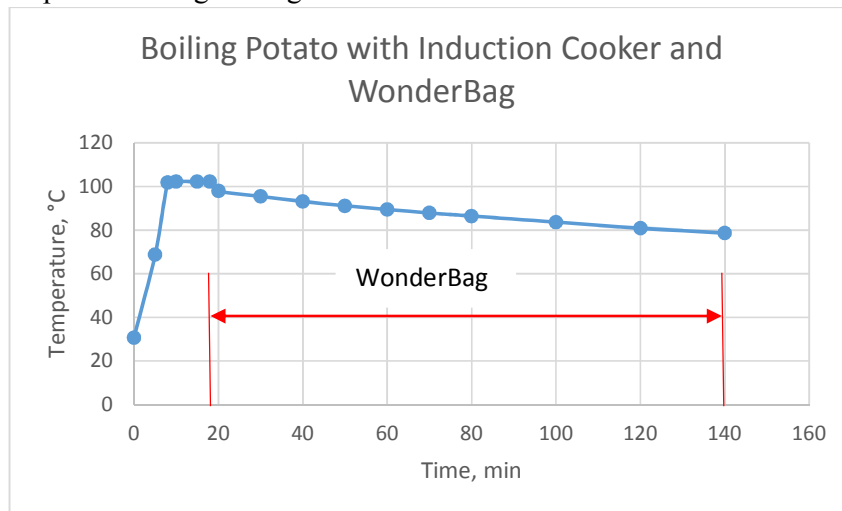
Fig.4.11 Boiling Potato with Induction Cooker and WonderBag
