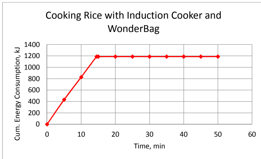
Fig. 5.2 Energy consumption profile for cooking rice with Induction Cooker and WonderBag
