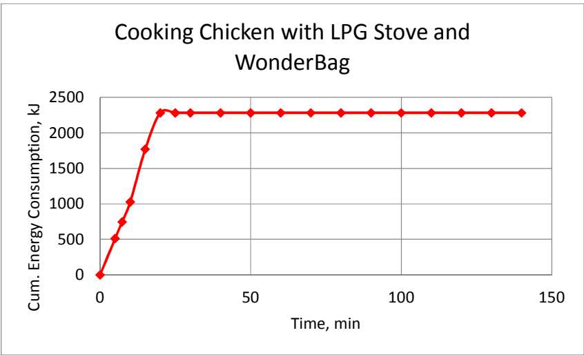
Fig.5.12 Energy consumption profile for cooking chicken with LPG Stove and WonderBag
