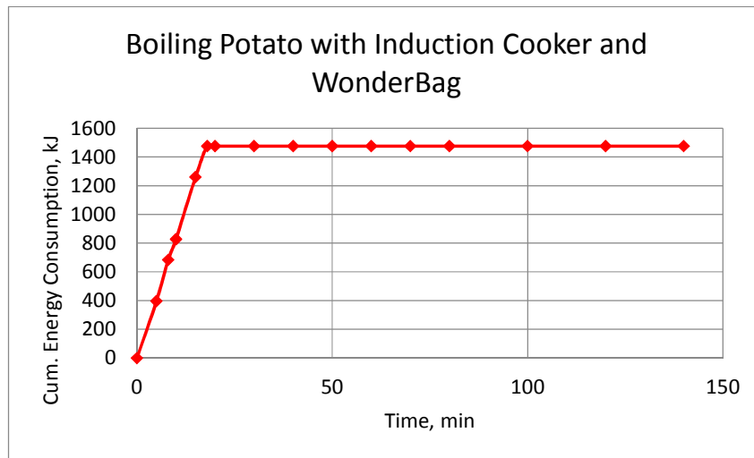
Fig.5.6 Energy consumption profile for boiling potato with Induction Cooker and WonderBag
