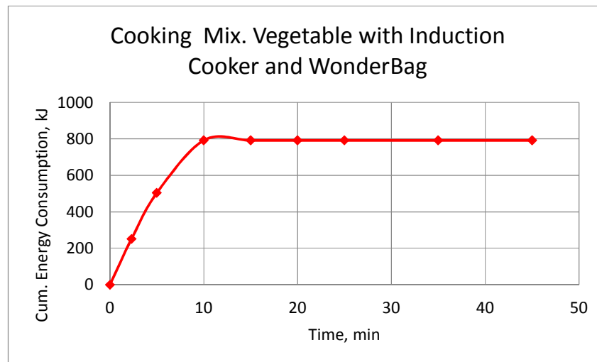
Fig.5.14 Energy consumption profile for cooking mix. Vegetables with Induction Cooker and WonderBag
