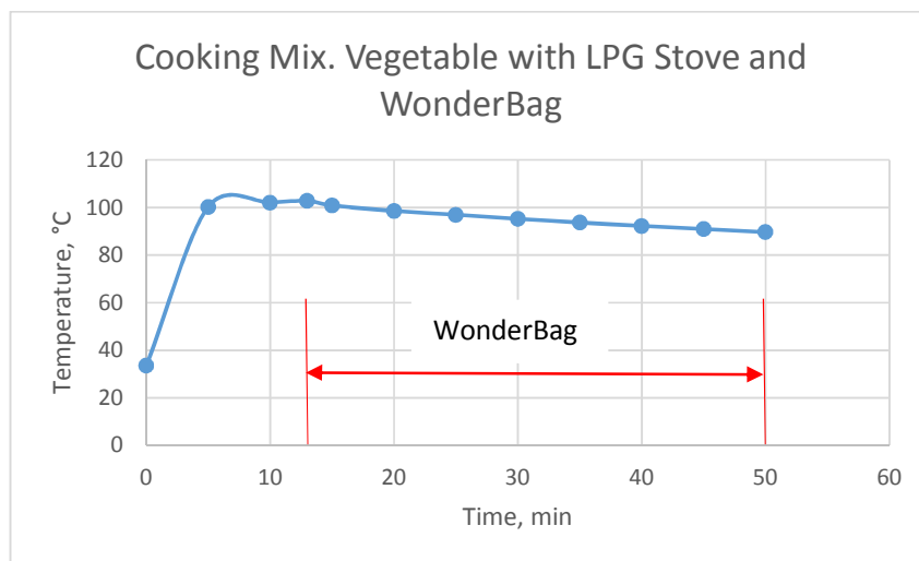
Fig. 4.26 Cooking Mix. Vegetable with LPG Stove and WonderBag
