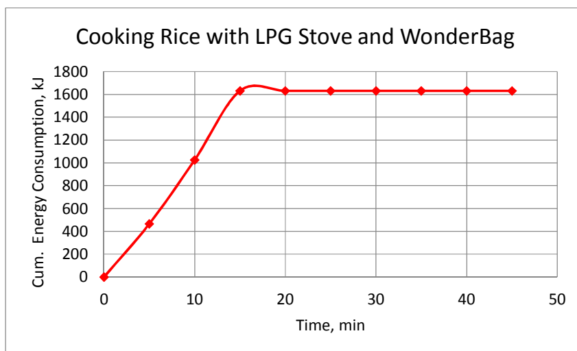
Fig.5.4 Energy consumption profile for cooking rice with LPG Stove and WonderBag
