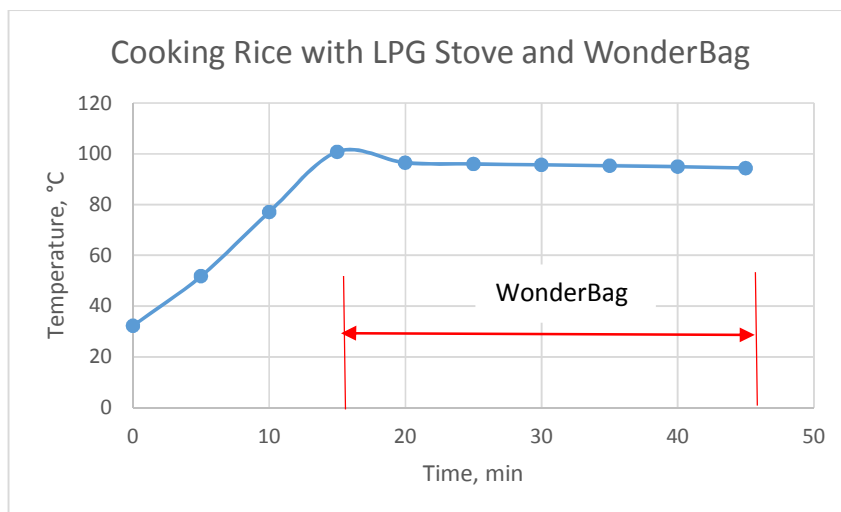
Fig. 4.8 Temperature profile for cooking rice with LPG Stove and WonderBag
