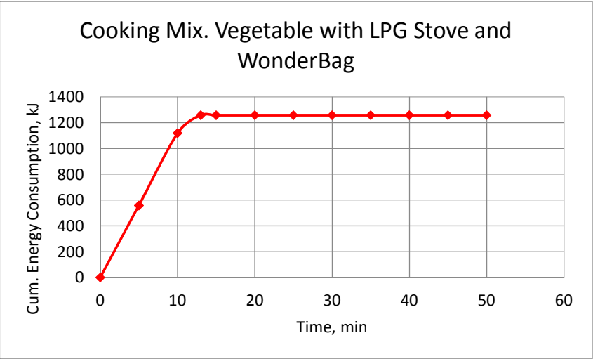
Fig.5.16 Energy consumption profile for cooking mix. Vegetables with LPG Stove and WonderBag
