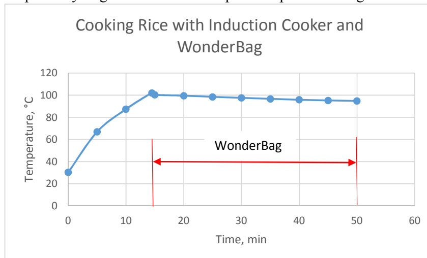
Fig. 4.6 Temperature profile for cooking rice with Induction cooker and WonderBag
