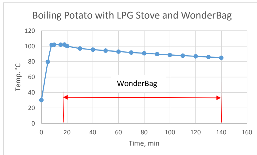
Fig.4.13 Boiling Potato with LPG Stove and WonderBag
