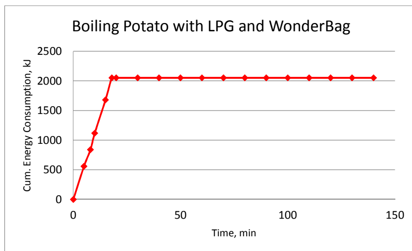
Fig.5.8 Energy consumption profile for boiling potato with LPG Stove and WonderBag
