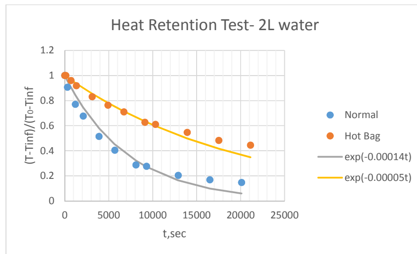
Fig. 6.9 Heat retention test for 2 liters water with and without WonderBag
