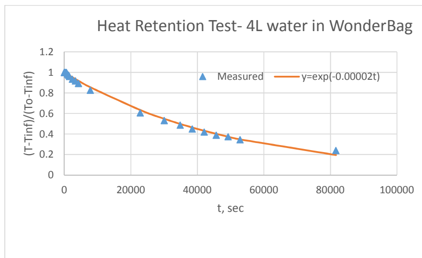
Fig. 6.7 Heat retention test for 4 liters with WonderBag
