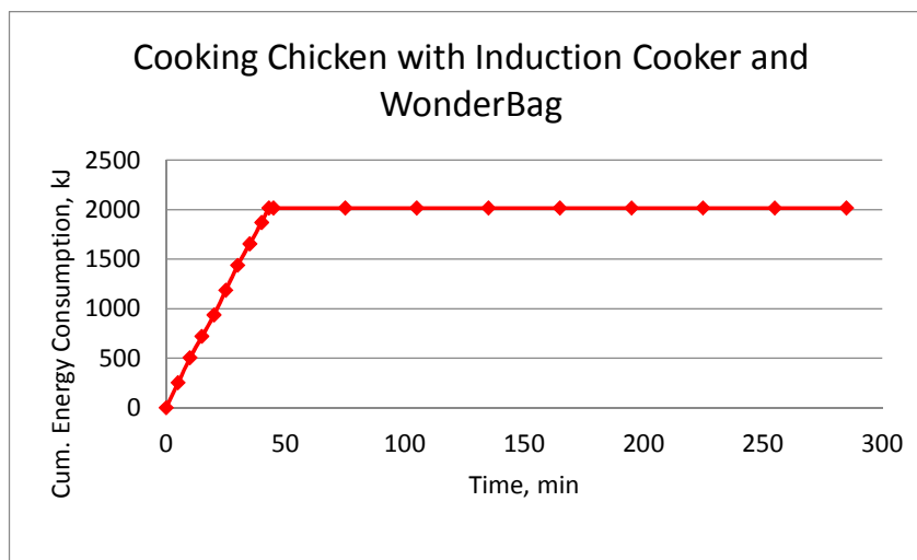
Fig.5.10 Energy consumption profile for cooking chicken with Induction Cooker and WonderBag
