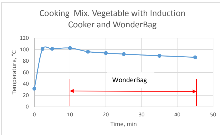
Fig.4.24 Cooking Mix. Vegetable with Induction Cooker and WonderBag
