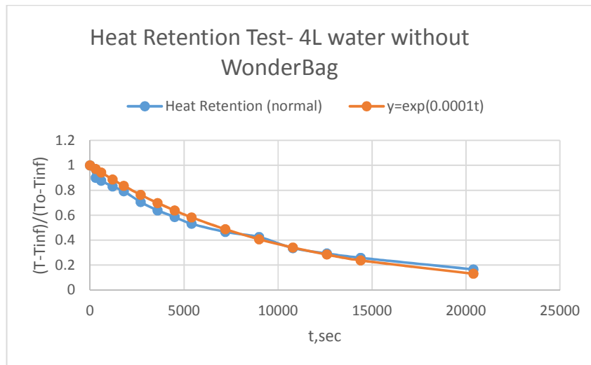
Fig. 6.8 Heat retention test for 4 liters without WonderBag
