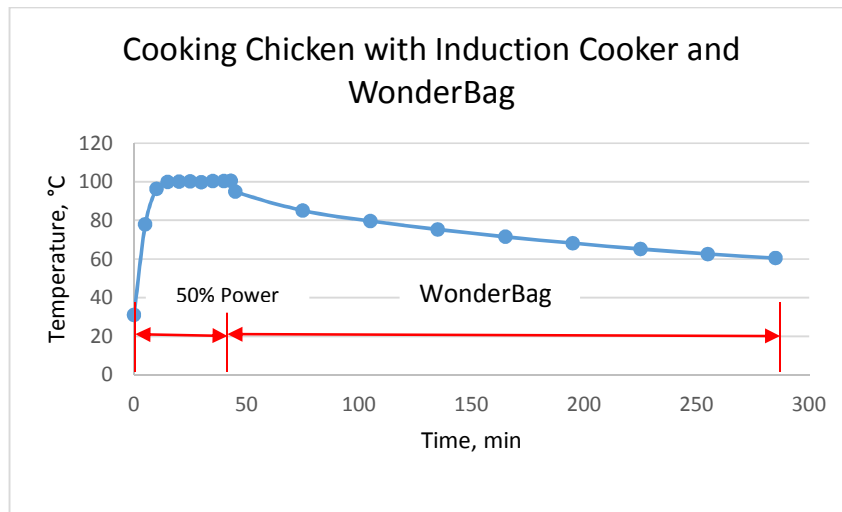
Fig.4.18 Cooking Chicken with Induction Cooker and WonderBag
