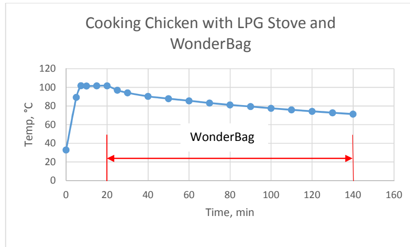
Fig. 4.20 Cooking Chicken with LPG Stove and WonderBag
