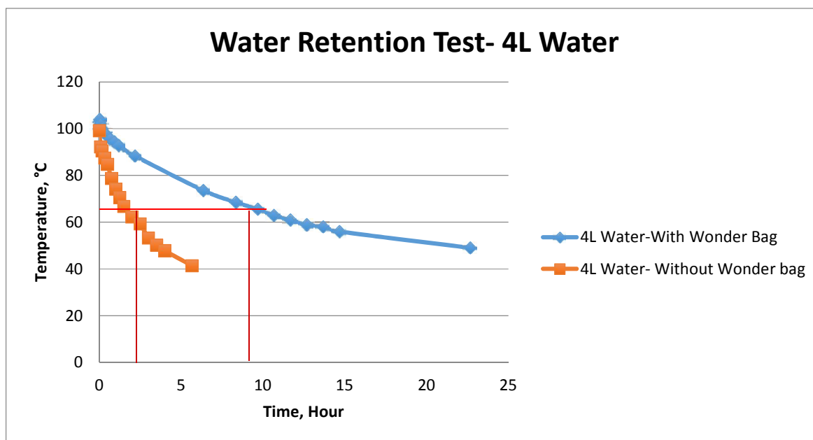
Fig. 3.9 Heat retention test for 4 liter water with and without WonderBag
