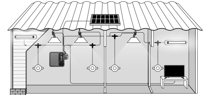
Example set-up of the BR!GHT Home 800 TV system
